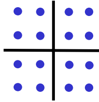
V.22bis 600 baud 2400 bps QAM
